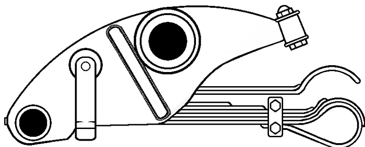
(bogie central.) - Central bogie. -
