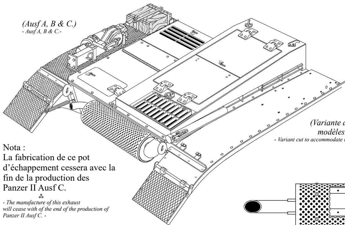
(Silencieux nu sans protection.) - Naked muffler without protection. -
